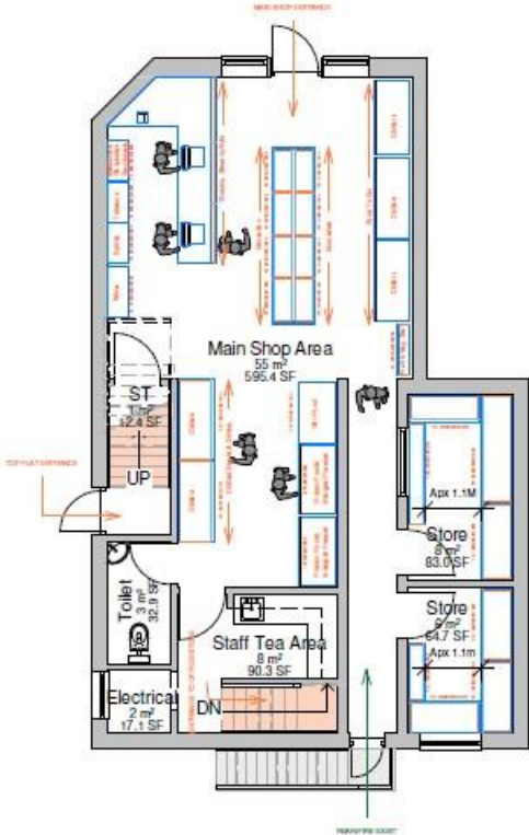
Ground Floor - Main Shop Area 1 : 100
